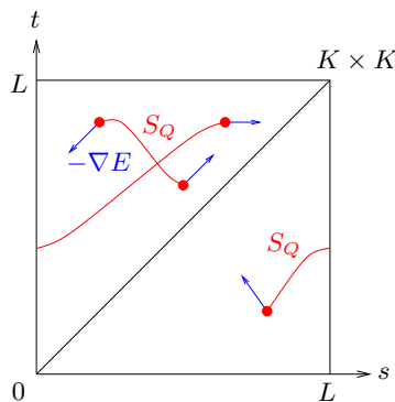
FIGURE 7.4. The space of 2-gons.
