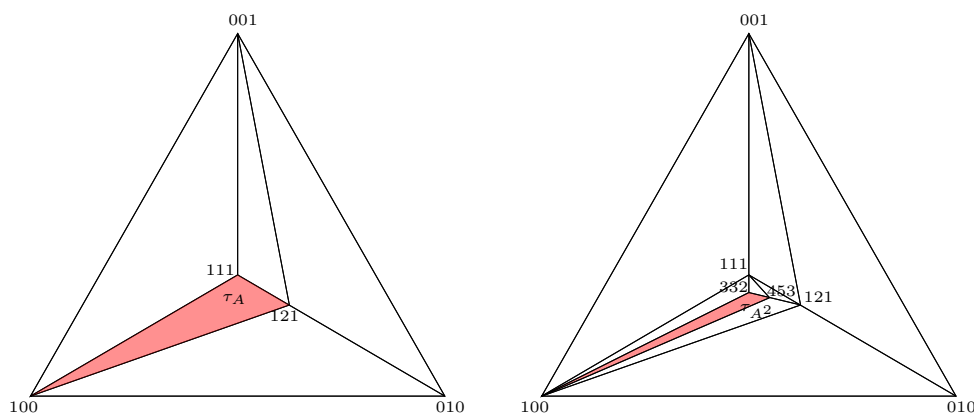
FIGURE 2. Toric Kato data with P(A) = \{1\} .
