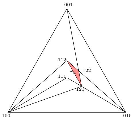
FIGURE 3. Fan associated to the toric modification \pi , invariant by the permutation Q of 9.11.
