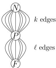
FIGURE 4. The graph \mathcal{G}(k,\ell) .
